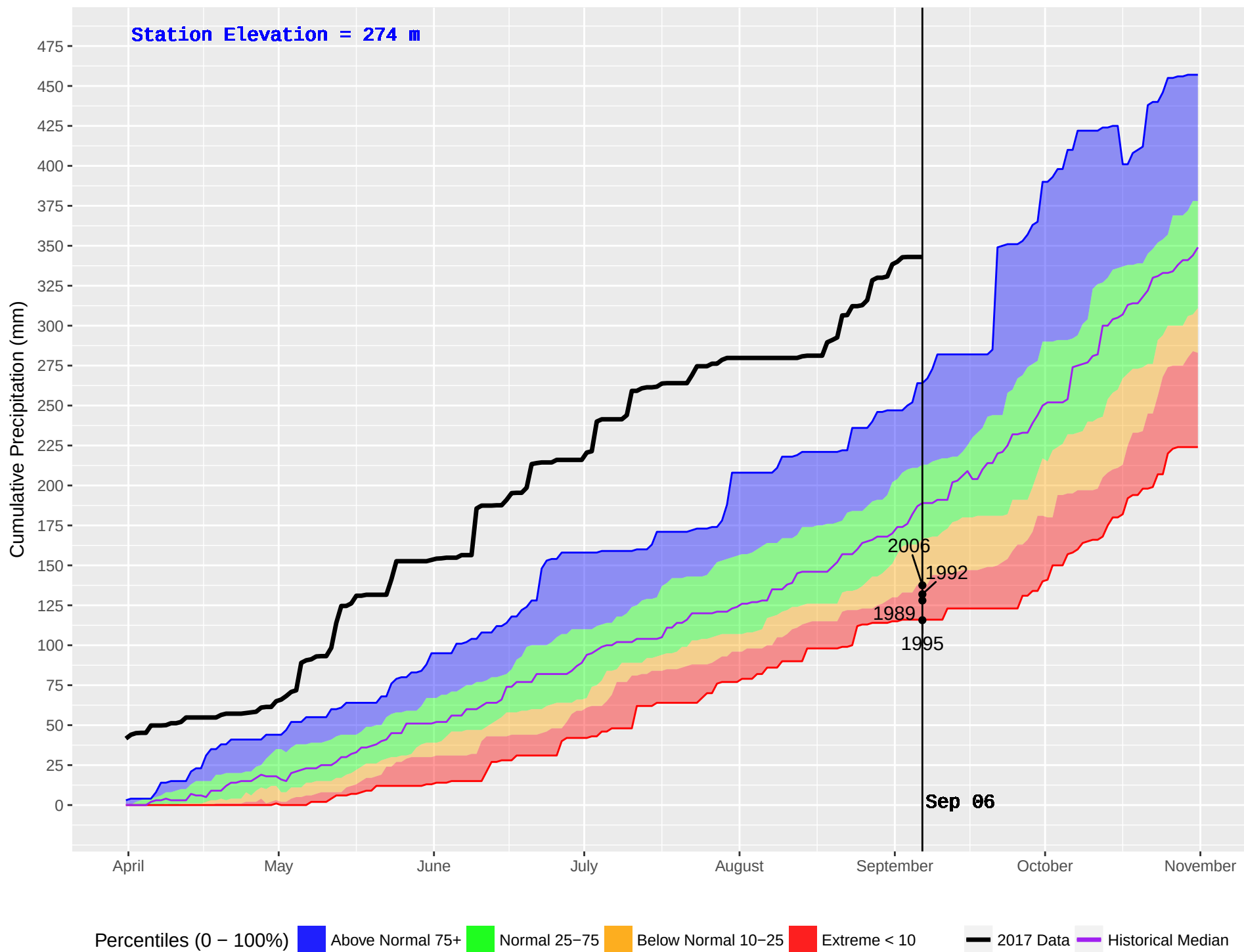
CEDARVALE (429) : Historical (1982–2016) and Current (2017) Noon Cumulative Precipitation
